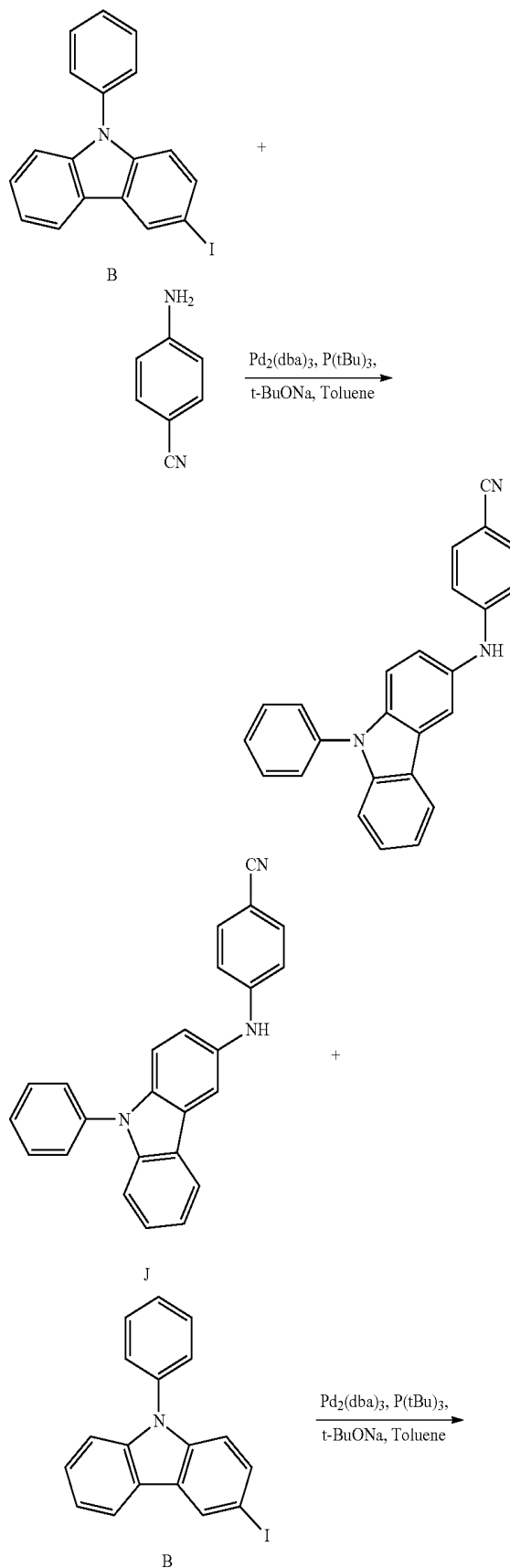
Reaction Scheme 8
